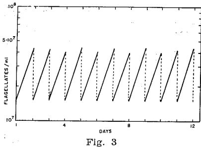
Fig. 3 — Permanent exponential growth of T. cruzi in LIT medium by daily subculturing. Initial concentration of flagellates: 15 \times 10^6 /ml.
