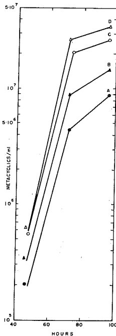
Fig. 4 — Growth in LAS medium. Initial concentrations (flagellates/ml) in cultures A, B, C and D were respectively 4.5 , 16.0 , 40.0 and 80.0 \times 10^6 .
